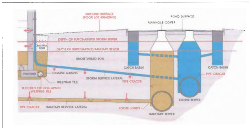
Storm sewer lateral
